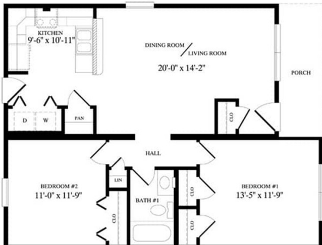
Annandale Duplex 27'-6" x 36'
